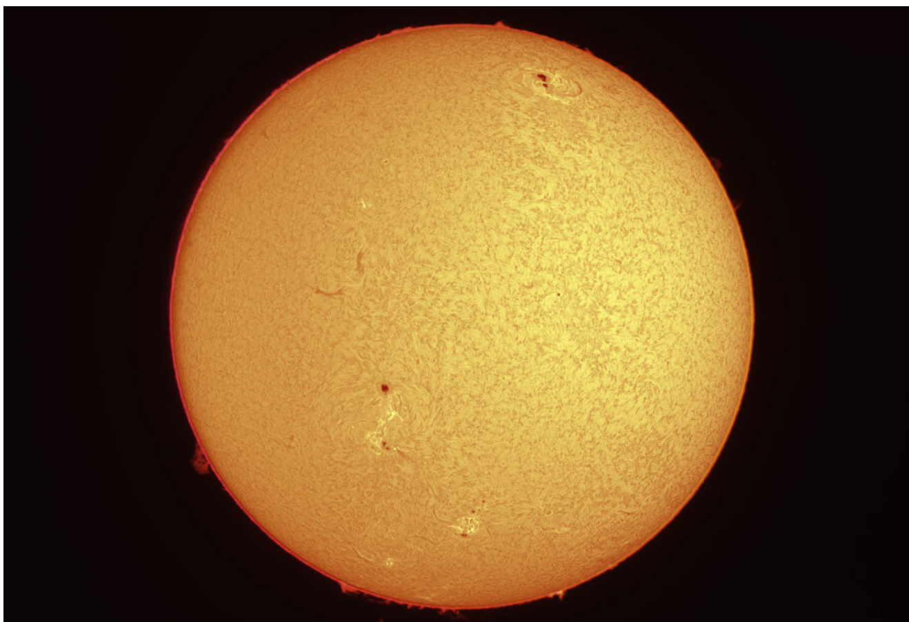
Sole in H \alpha - 16/07/2023
